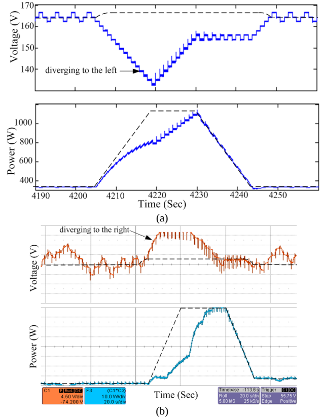
Fig. 9. The tracking performance of the conventional P&O for the 50 W/m 2 ramp; (a) simulation (b) experimental
