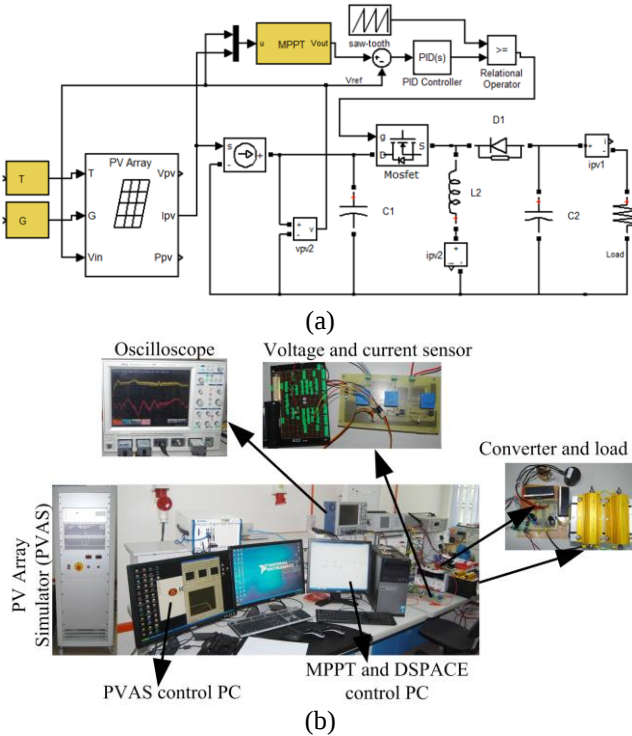
Fig. 5. (a) The Matlab simulation platform (b) The Hardware setup
