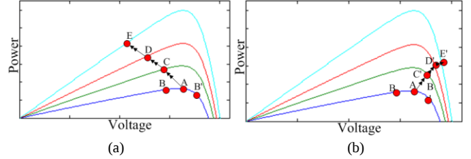
Fig. 1. The losing of the tracking direction by conventional P&O (a) towards the left (b) towards the right of the P - V curve.
