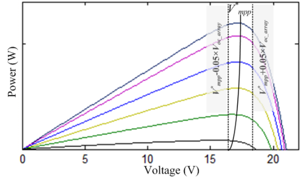
Fig. 3. The position change of V_{MPP} depending of the irradiance level
