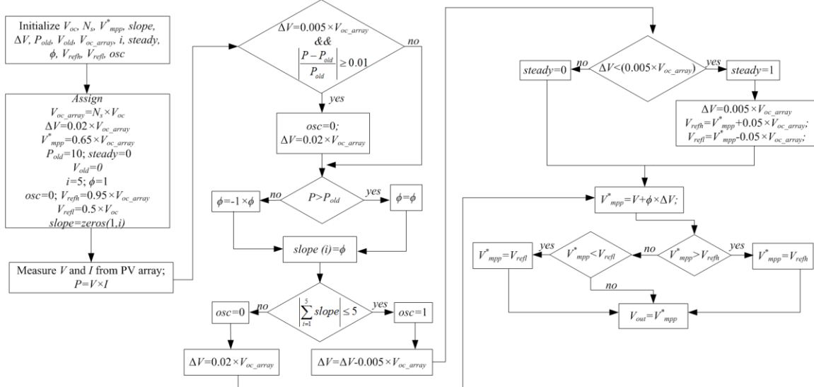
Fig.4. The complete flowchart of the Modified P&O
