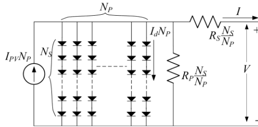
Fig. 2. The two-diode model with the series-parallel combination
