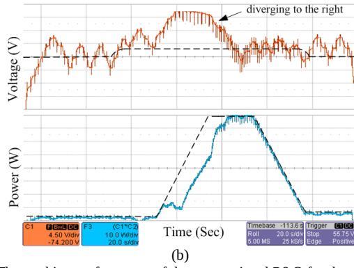
Fig. 7. The tracking performance of the conventional P&O for the 30 W/m 2 ramp; (a) simulation (b) experimental
