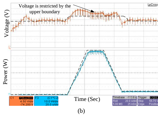
Fig. 10. The tracking performance of the modified P&O for the 50 W/m 2 ramp; (a) simulation (b) experimental
