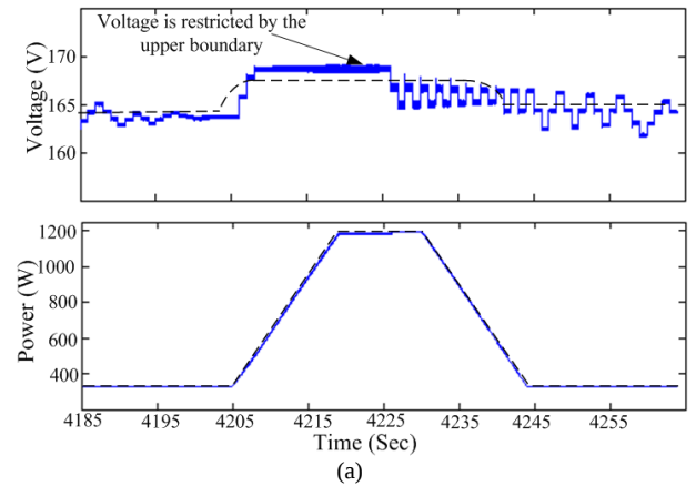
Fig. 9. The tracking performance of the conventional P&O for the 50 W/m 2 ramp; (a) simulation (b) experimental
