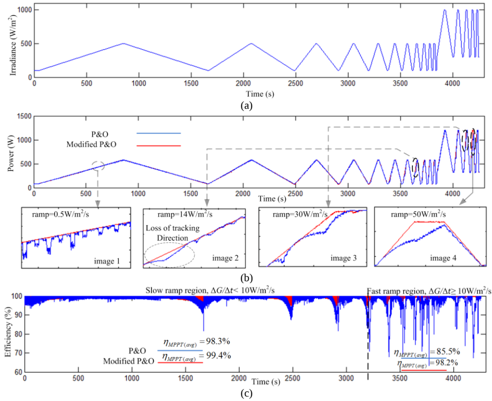
Fig. 6. (a) The irradiance profile for the EN50530 test (b) The tracking performance of the conventional P&O and the modified P&O (c) Efficiency of the conventional P&O and the modified P&O
