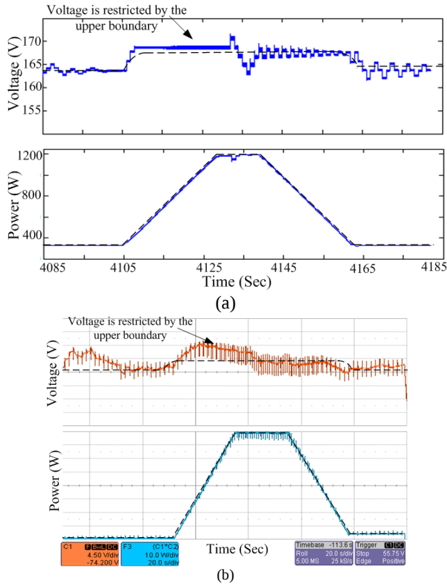
Fig. 8. The tracking performance of the modified P&O for the 30 W/m 2 ramp; (a) simulation (b) experimental
